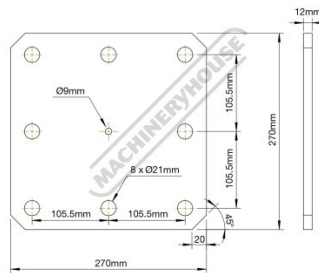
Base Dimensions
