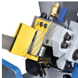
Ball Bearing Blade Guides Back
