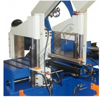
Hydraulic Hitch Feed With Bundle Cutting Clamps
