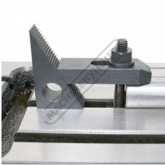
Shown Setup
