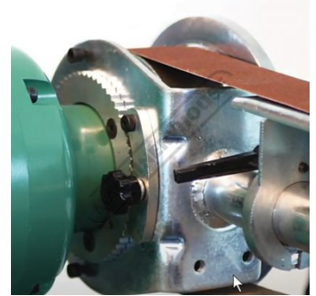
Quick Action Lock To Adjust Linisher Angle
