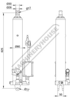
Drawing Dimensions
