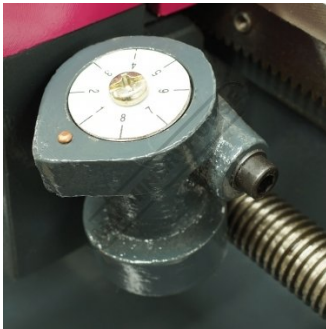
TU 2506V Thread Chasing Dial
