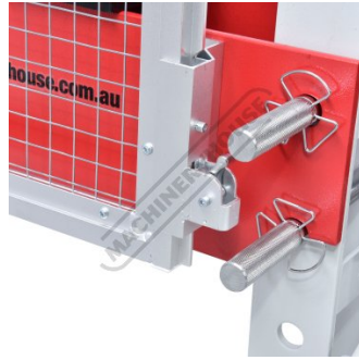
Safety Guard Quick Release with Table Height Adjustment With Safety Clips
