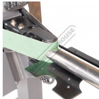
Pipe Notching
