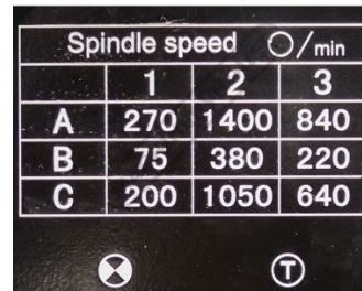
Spindle Speed Chart
