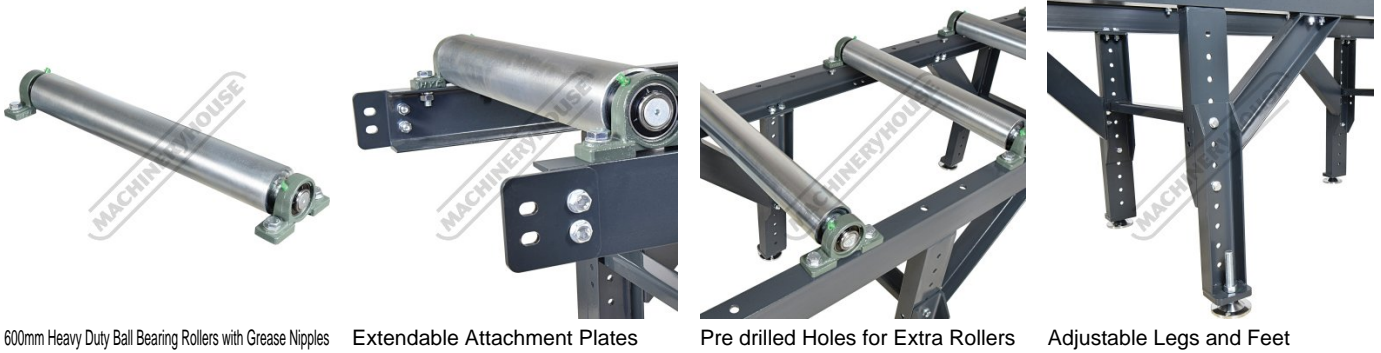
600mm Heavy Duty Ball Bearing Rollers with Grease Nipples
