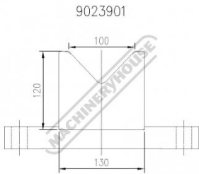
Single Vee Pressbrake Diagram
