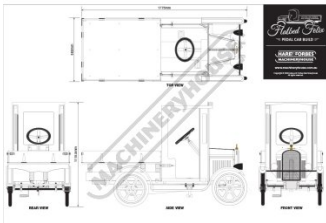
Dimensions of Finished Pedal Car
