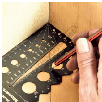
Marking Angles
