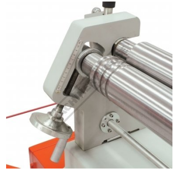
Curving Roller Height Adjustment
