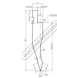
Segmented Top Punch
