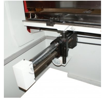
Ezy Set NC 89 Control with Ballscrew Backgauge
