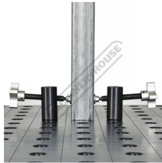
Clamp Position
