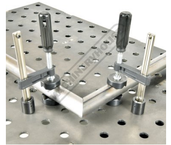
Round Tube Setup with Clamps and Optional V Pads
