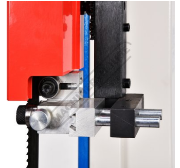
Adjustable Ball Bearing Blade Guides
