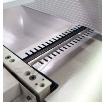
3 Blade Cutter Head
