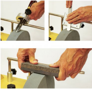
W8625 Jig 55, 110 & Stone Grader Wood Turners Sharpening Kit - 3 Piece Set
