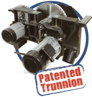
Trunnion
